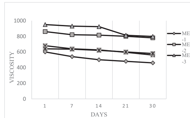
Figure 6. Graph of base microemulsion viscosity values.
