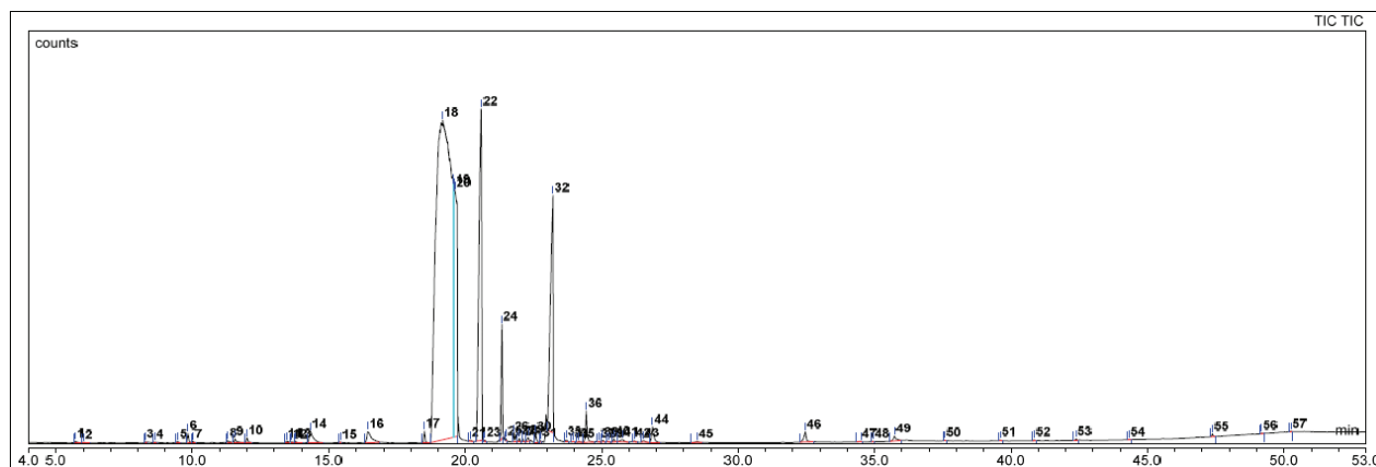
Figure 1. The chromatogram profile of clove essential oil.
