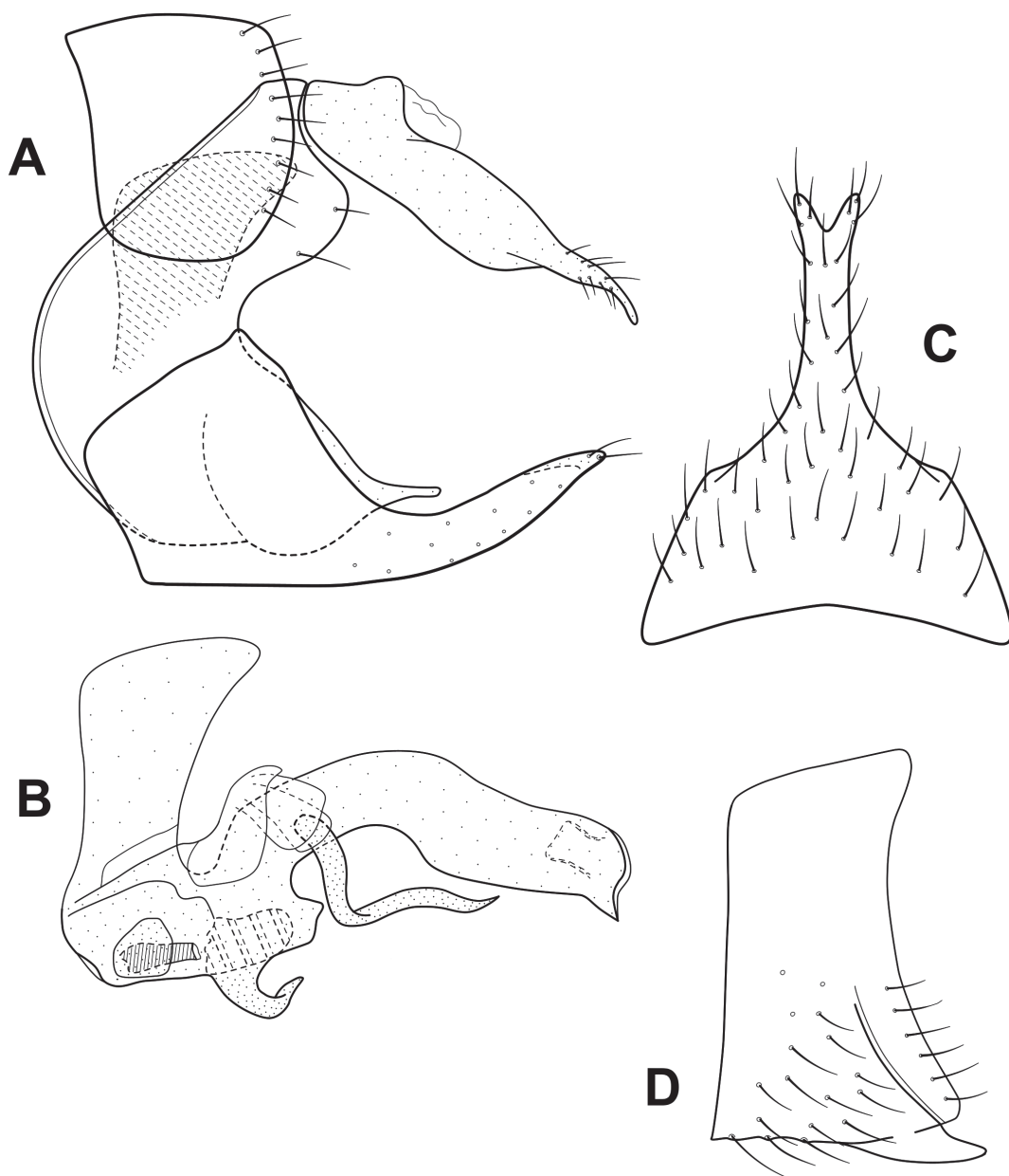
Figure 2. Protophila harrisi , sp. nov., male genitalia A lateral (position of phallic apparatus in genital capsule indicated with cross hatches B phallic ensemble, lateral C sternum VIII, ventral D sternum VI, ventral process, lateral.
