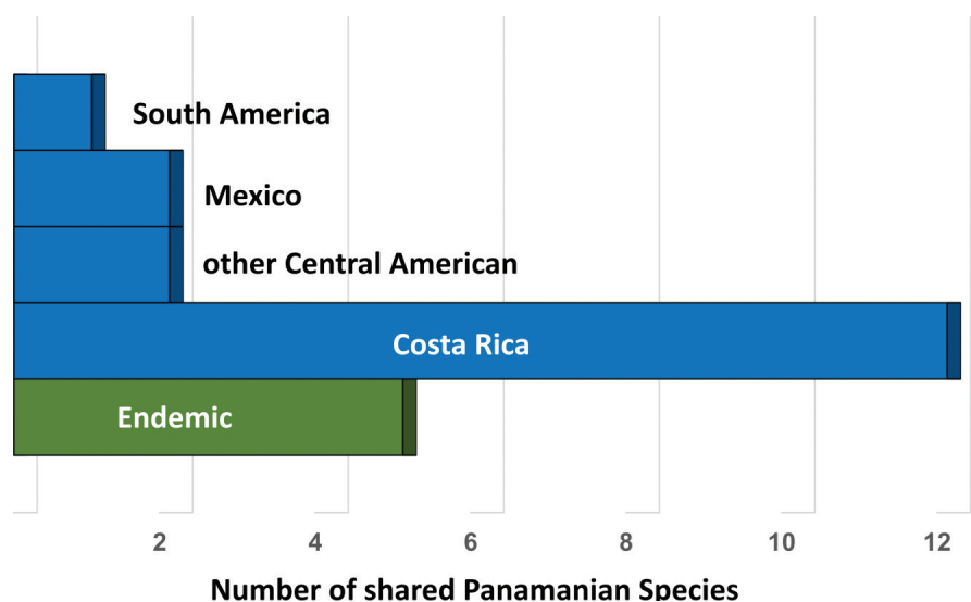
Figure 3. Number of Panamanian species of Protoptila shared with other country or regional areas.
