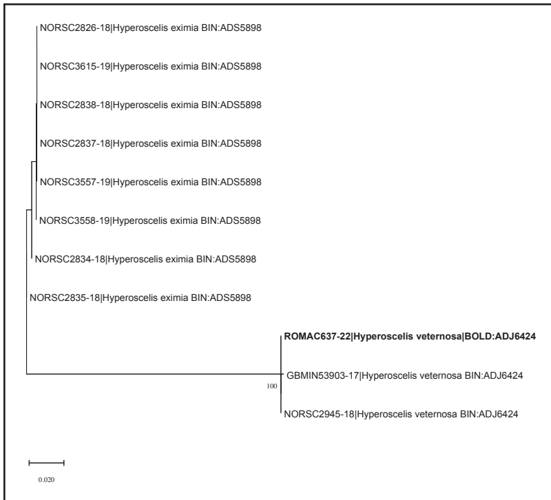
Figure 3. NJ-tree (Kimura-2-distance) with all barcodes available for the European Canthyloscelidae fauna, with their associated BIN numbers. The single specimen collected by us is marked in bold.
