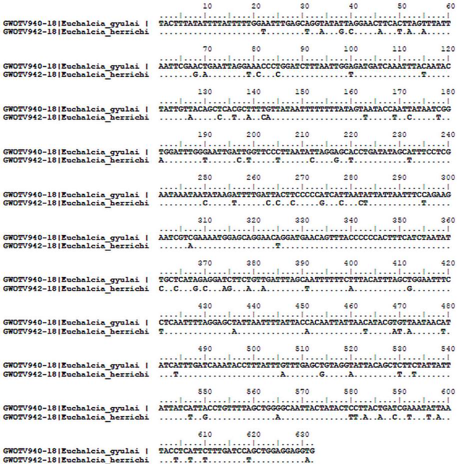
Figure 1. Alignment of the COI sequences of Euchalcia gyulai and E. herrichi
