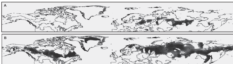
Figure 3. The model of the suitable area for Brunnera sibirica , in Eurasia in accordance with the bioclimatic variables Bio 2, 7, 8, 9, 15, 18, 19. The names of bioclimatic characteristics are in the text. A – current climate. B – climate, predicted by SCIRO for 2080 (emission scenario A2a).
