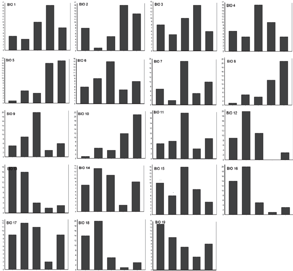
Figure 2. Variability of various climatic characteristics (Bio 1 – Bio19) of Brunnera sibirica . The names of bioclimatic characteristics are in the text. (Axis of abscissa – the factor strength, ordinate axis – the frequencies).
